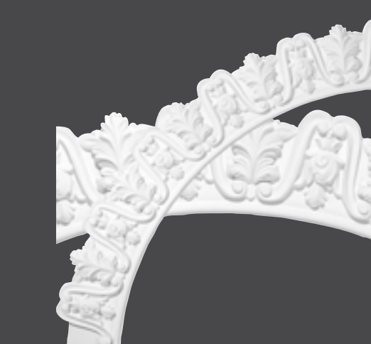
Product ID OD ID W P CR57TI 57 3/8" 46 1/8" 5 5/8" 1"
