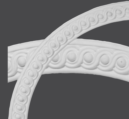
Product ID OD ID W P CR41HI 40 1/4" 34" 3 1/8" 3/4"
